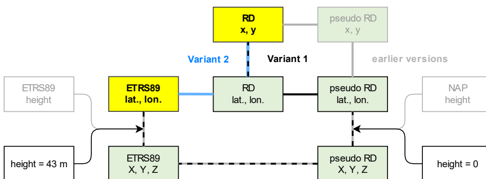
Figure 1.2.1. Transformation procedure of RDNAPTRANS™2018 implementation variant 1 (black lines) and implementation variant 2 (blue lines) compared to RDNAPTRANS™2008 and earlier versions (grey lines).
