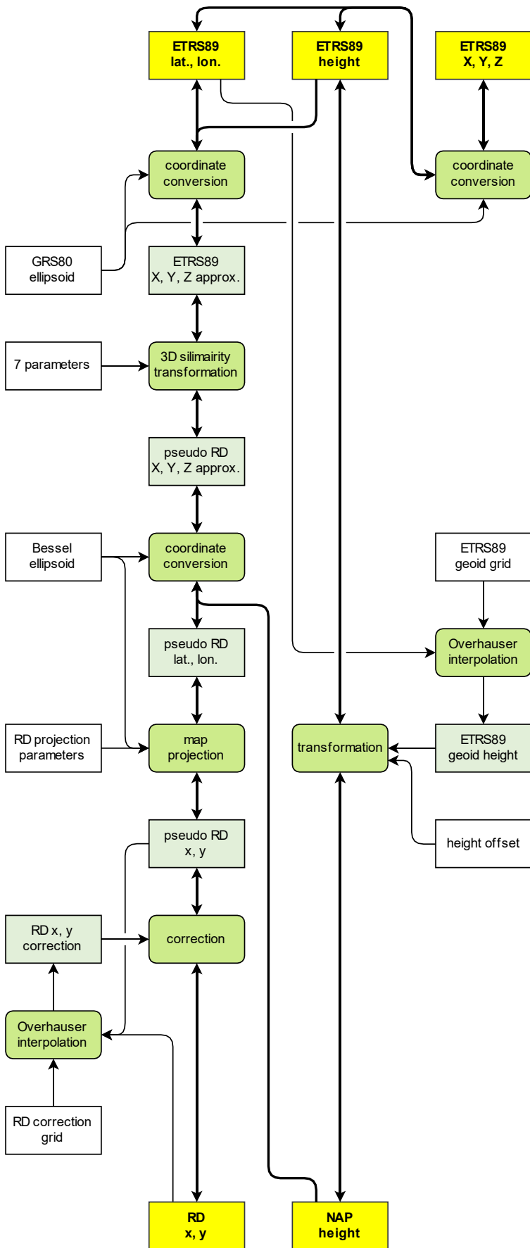
Figure A1.3. Transformation procedure of RD NAPTRANS TM 2008 (official variant) and earlier versions of RD NAPTRANS TM .
